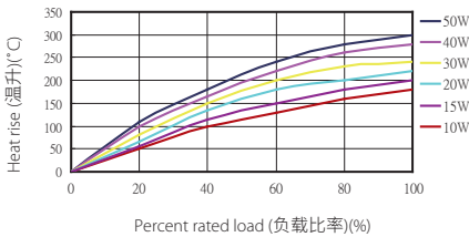
Radial Terminal Type - PRT (With metal mounting bracket)/PRU Series
