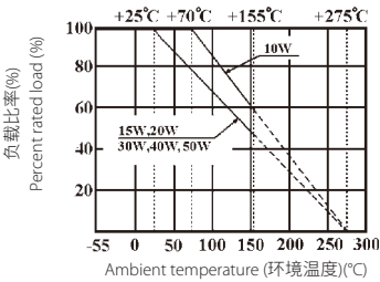
Radial Terminal Type - PRT (With metal mounting bracket)/PRU Series
