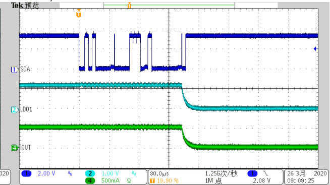
LDO1, IOUT=500mA
