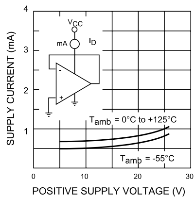
Figure 14. Supply current
