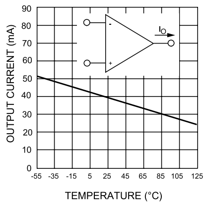
Figure 12. Current limiting
