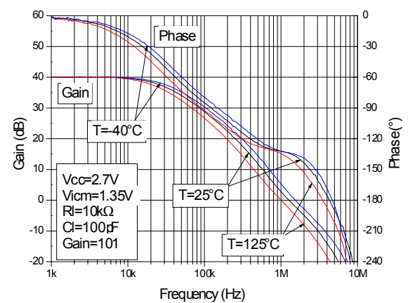
Figure 17. Bode diagram at V_{CC} = 2.7\text{ V}
