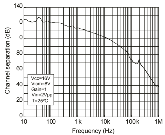
Figure 5. Channel separation
