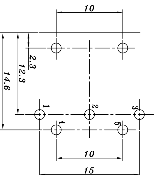
PCB LAYOUT
