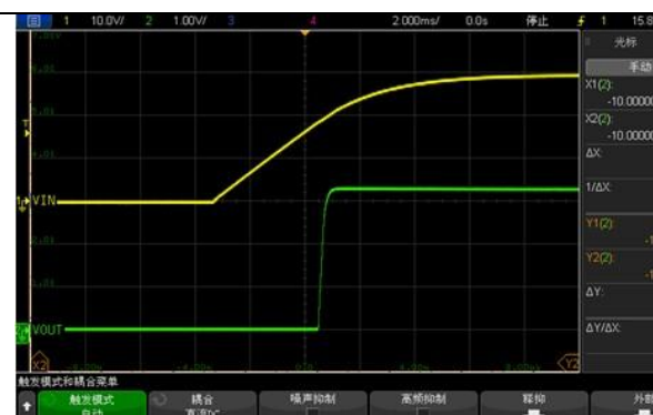
Vin=30V, Iout=30mA, Cout=10uF
