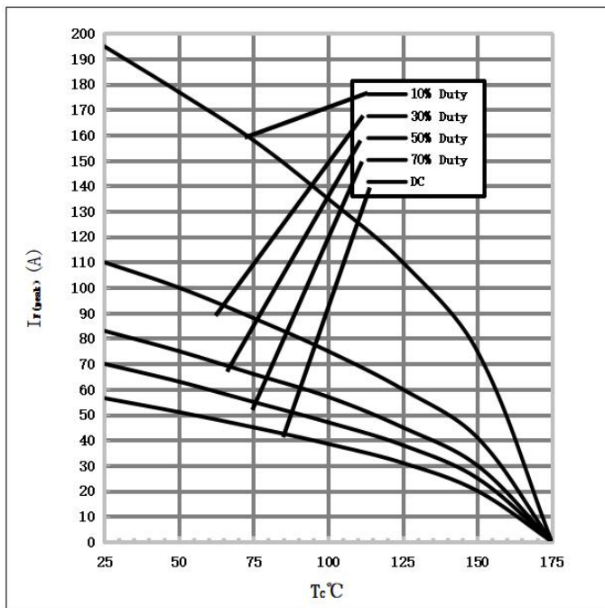
Figure 3. Current Derating
