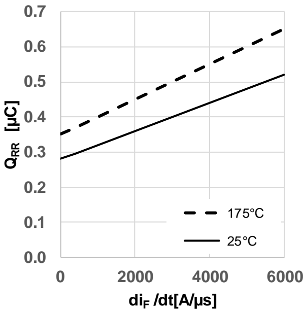
Figure 19 Typical reverse recovery charge as a function of diode current slope ( Q_{rr} = f(di_i/dt) , V_{DD} = 800V , V_{GS} = 0V/18V , I_D = 25A , ind. load, test circuit in Fig.E, body diode at V_{GS} = 0V )
