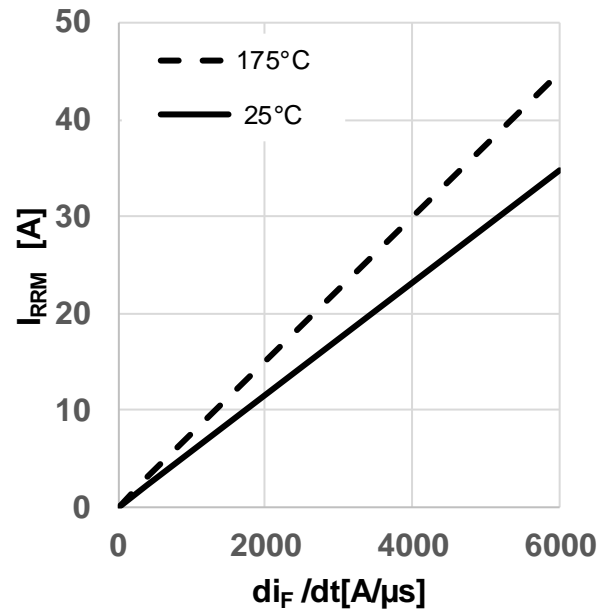
Figure 20 Typical reverse recovery current as a function of diode current slope ( I_{rrm} = f(di_i/dt) , V_{DD} = 800V , V_{GS} = 0V/18V , I_D = 25A , ind. load, test circuit in Fig.E, body diode at V_{GS} = 0V )
