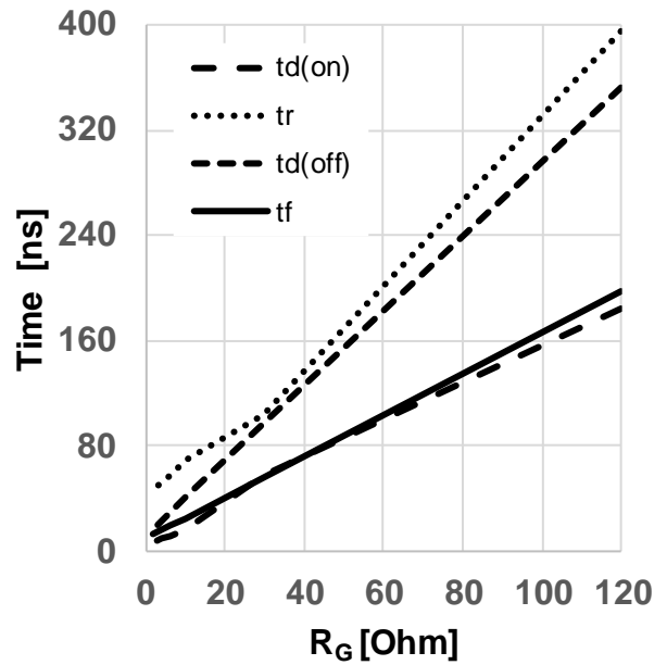
Figure 18 Typical switching times as a function of gate resistor ( t = f(R_{G,ext}) , V_{DD} = 800V , V_{GS} = 0V/18V , I_D = 25A , T_{vj} = 175^{\circ}C , ind. load, test circuit in Fig. E, diode: body diode at V_{GS} = 0V )
