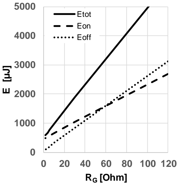
Figure 17 Typical switching energy losses as a function of gate resistance ( E = f(R_{G,ext}) , V_{DD} = 800V , V_{GS} = 0V/18V , I_D = 25A , T_{vj} = 175^{\circ}C , ind. load, test circuit in Fig. E, diode: body diode at V_{GS} = 0V )
