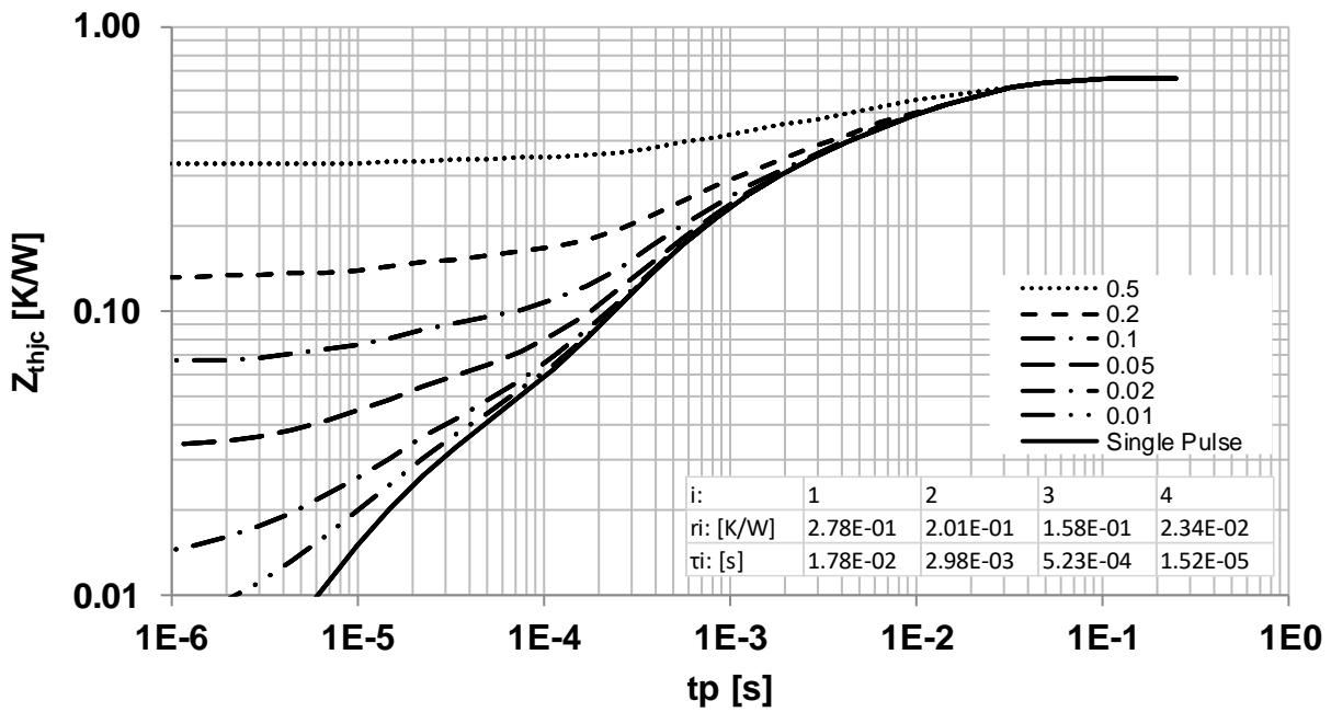
Figure 21 Max. transient thermal resistance (MOSFET/diode) ( Z_{th(j-c,max)} = f(t_p) , parameter D = t_p/T , thermal equivalent circuit in Fig. D)
