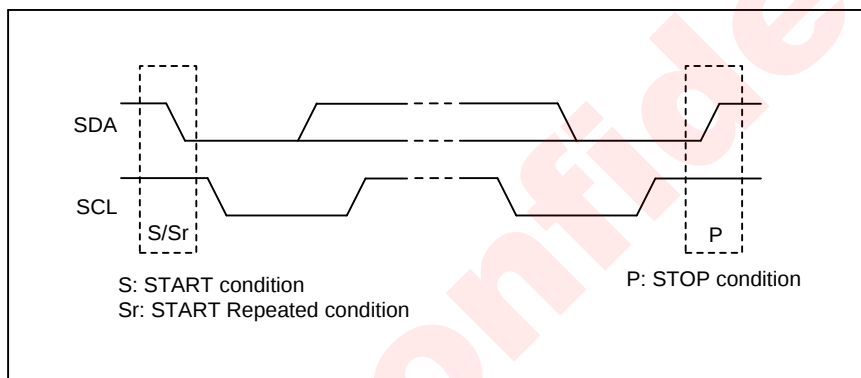
Figure 9 I²C Start/Stop Condition Timing
