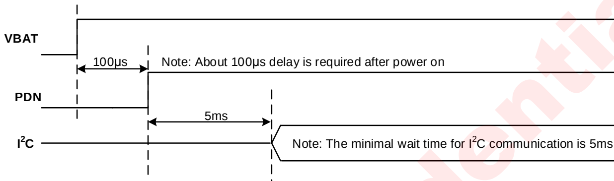
Figure 4 AW9109 Power On
