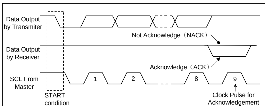
Figure 8 I²C ACK Timing
