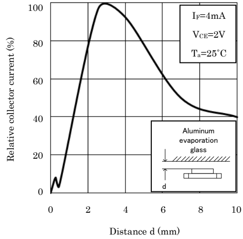
Fig.8 Relative Collector Current vs. Distance
