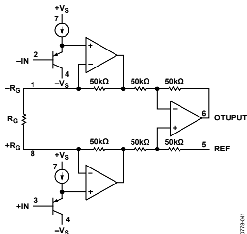
Figure 41. Simplified Schematic
