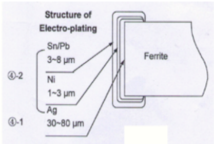
-1 Terminal electrode:Inside(Ag) -2 Outside (Electro-plating Ni-Sn/Pb)
