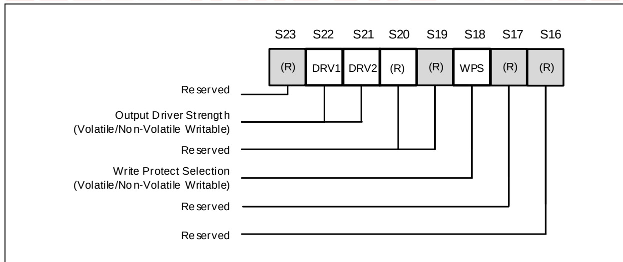
Figure 4c. Status Register-3
