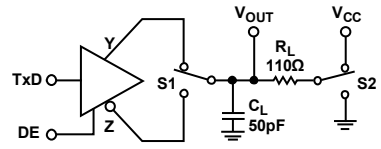
Figure 26. Driver Enable/Disable
