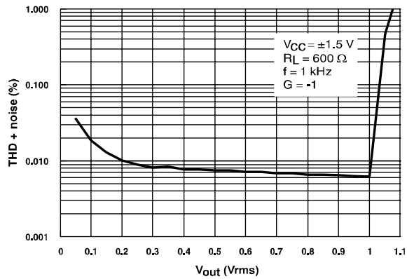
Figure 7: THD + noise vs. V_{out} ( V_{CC} = \pm 1.5\text{ V} , R_L = 600\ \Omega , f = 1\text{ kHz} , G = -1 )
