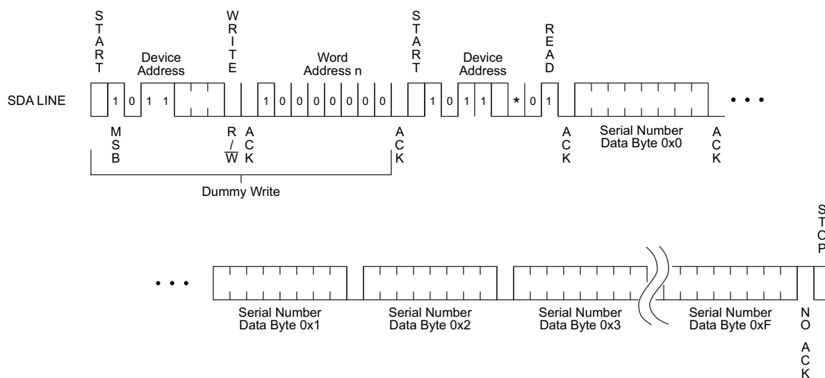
Figure 10-4. Serial Number Read
